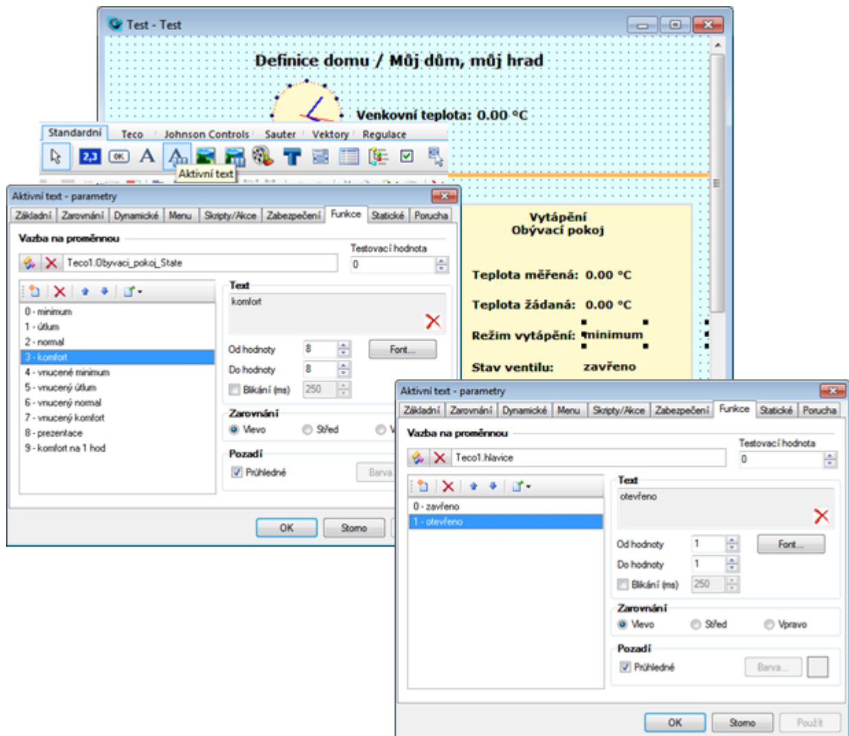
Picture No. 16 - Visualization and control of a heating circuit
