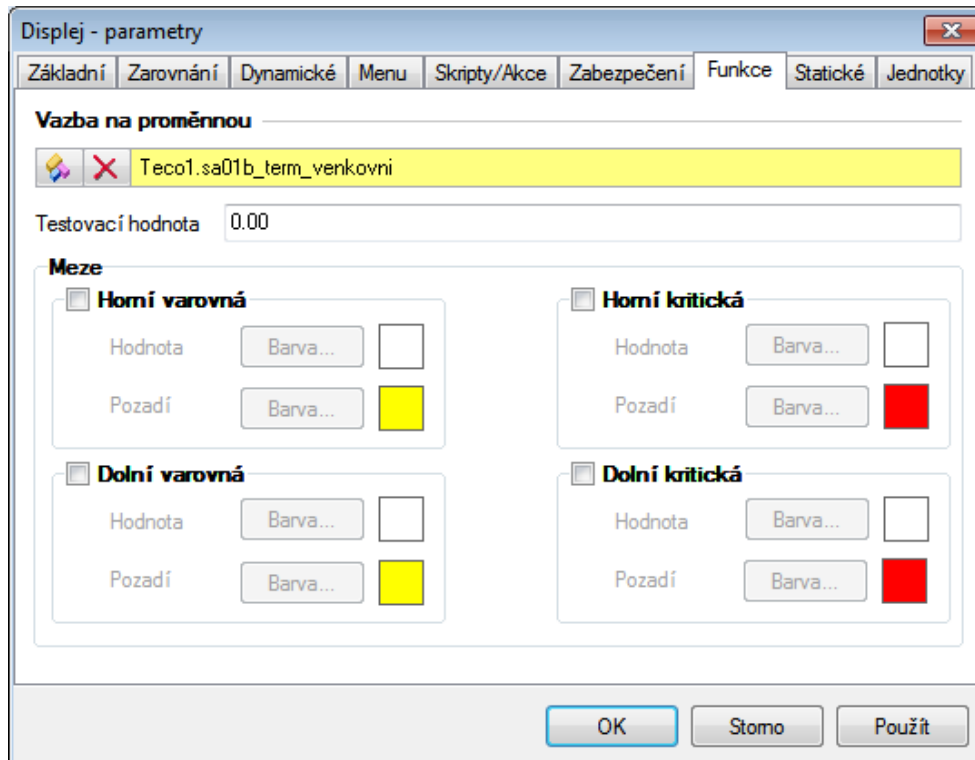
Picture No. 12 - Display component - Properties - Functions (Link to tag)
