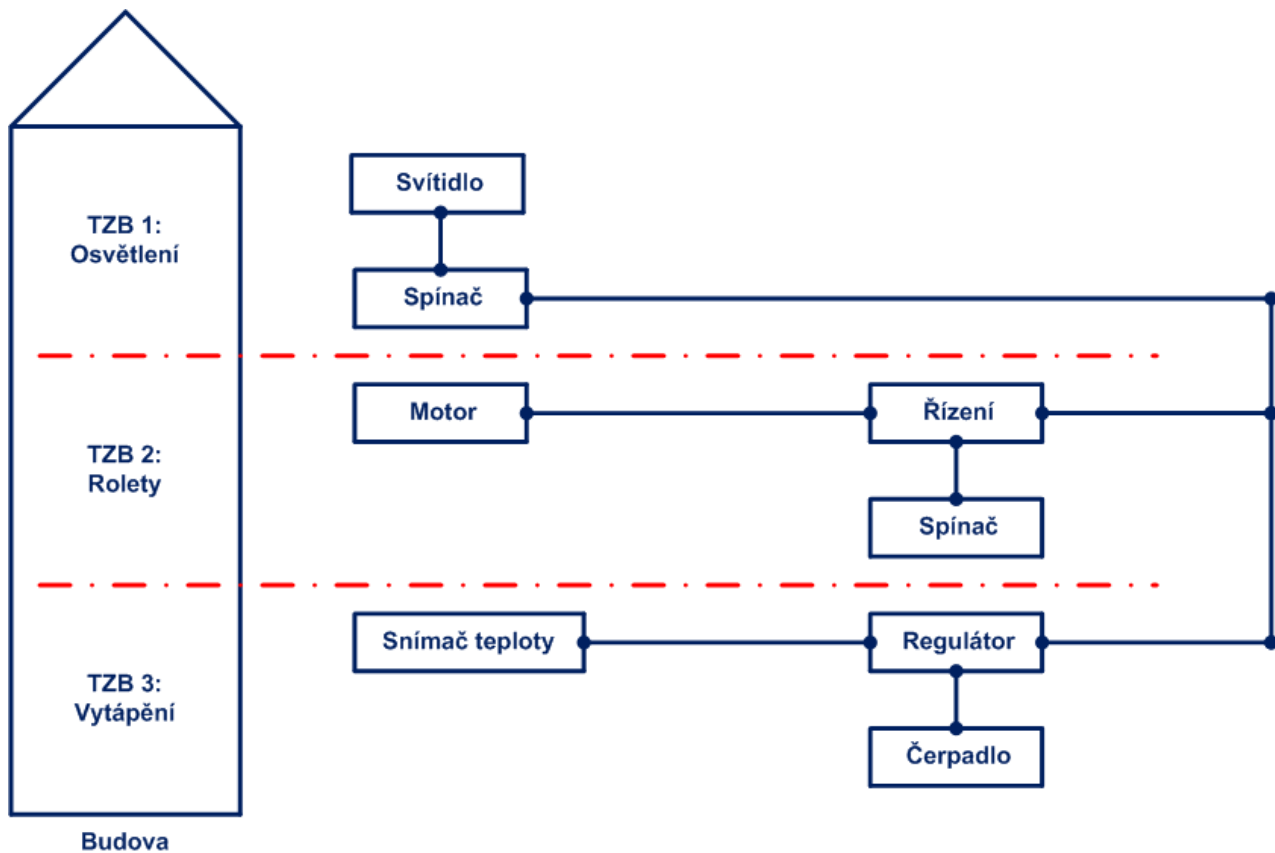
Picture No. 2 - Conventional wiring
