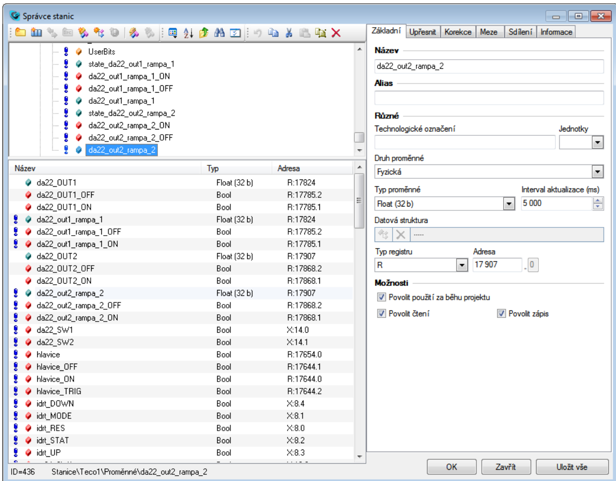
Picture No. 8 - Device Manager - List of imported tags
